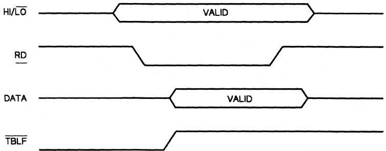
Figure 3-29. External Read Timing from the Coprocessor Port
