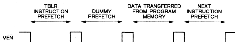
Figure 3-17. TBLR Instruction Timing
