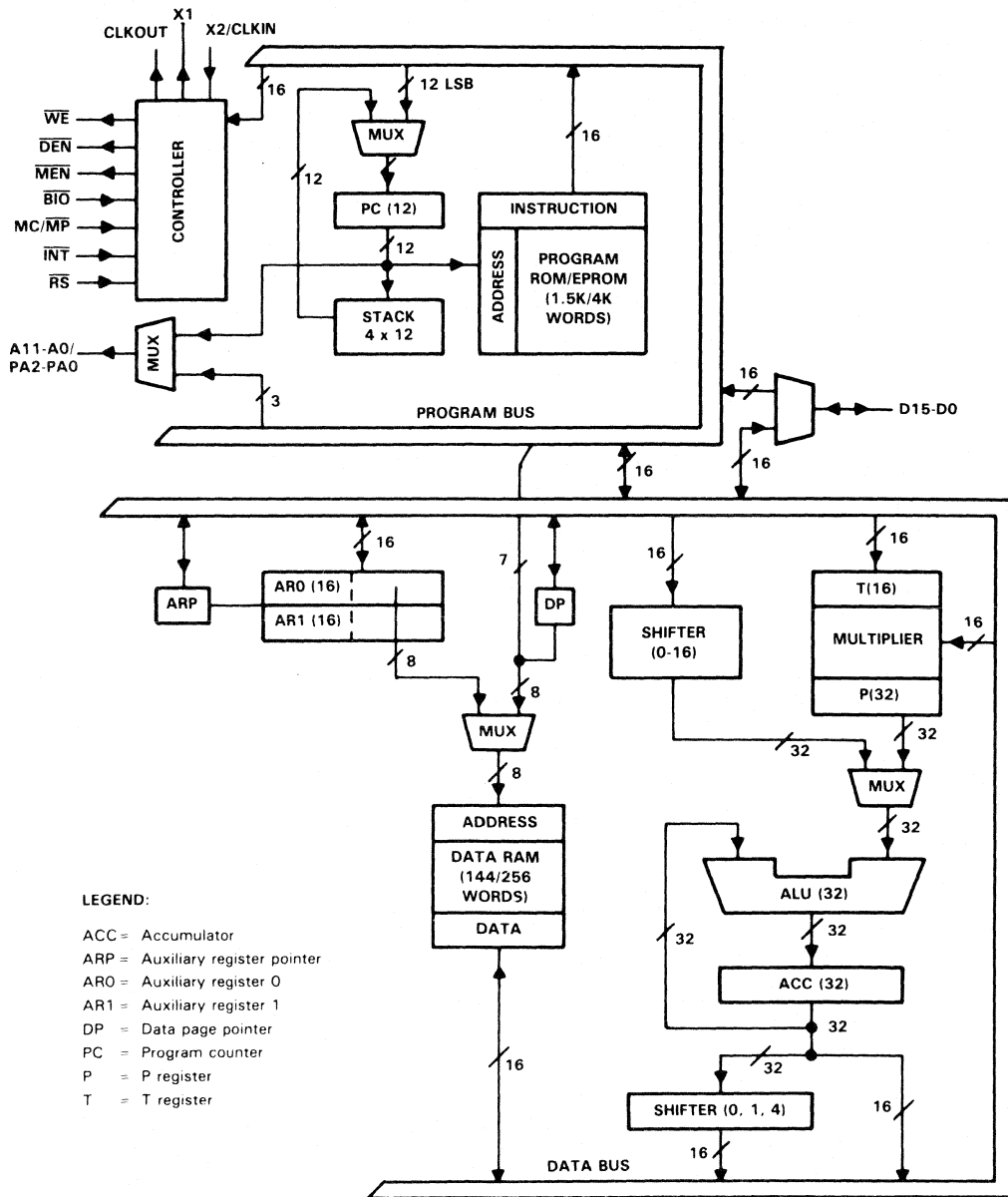
functional block diagram (TMS32010, TMS320C10, TMS320C15, TMS320E15)
