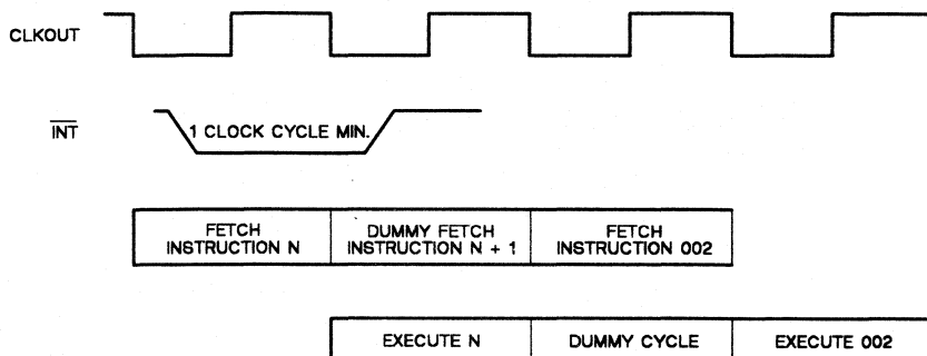
Figure 3-20. Interrupt Timing
