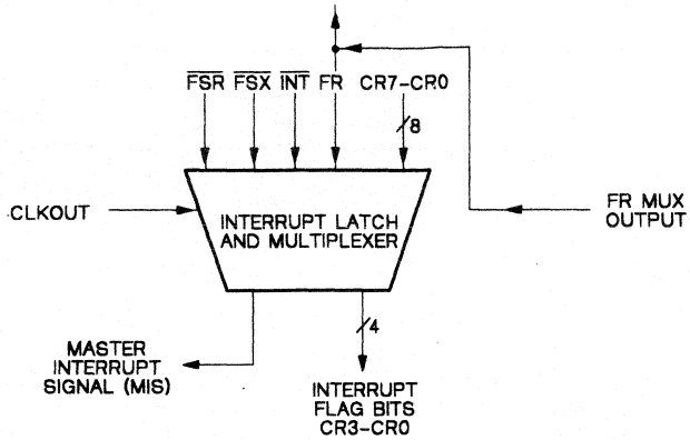
Figure 3-21. Interrupt Latch and Multiplexer
