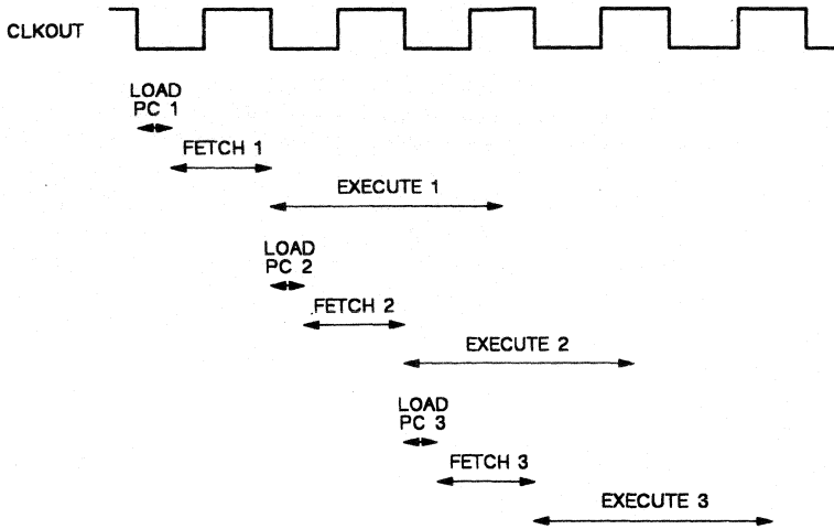
Figure 3-12. Harvard Architecture
