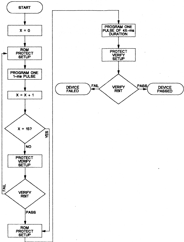
Figure G-5. ROM Protect Flowchart
