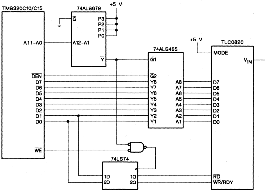
Figure 6-5. A/D Converter to TMS320C10/C15 Interface
