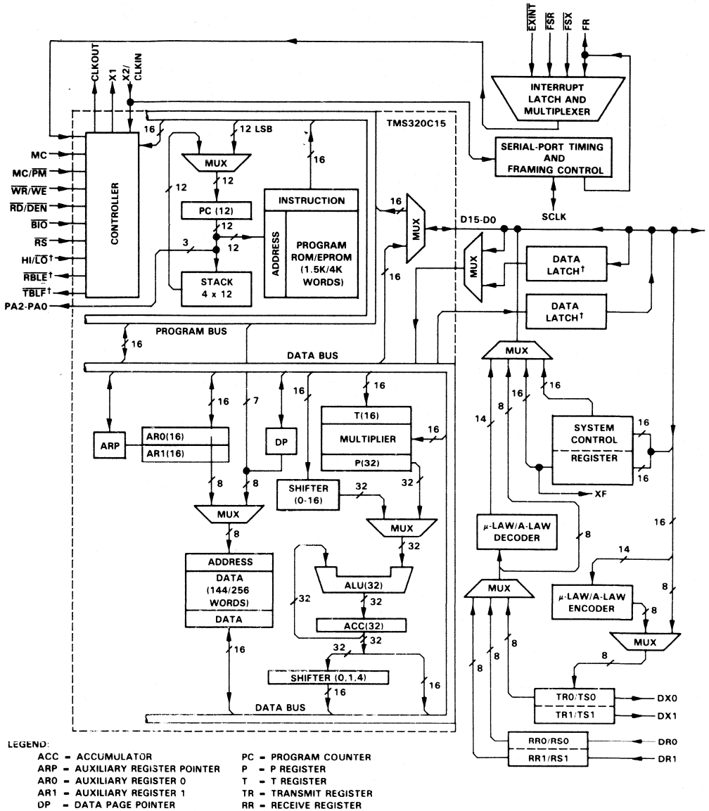
Figure 3-2. TMS320C17/E17 Block Diagram
