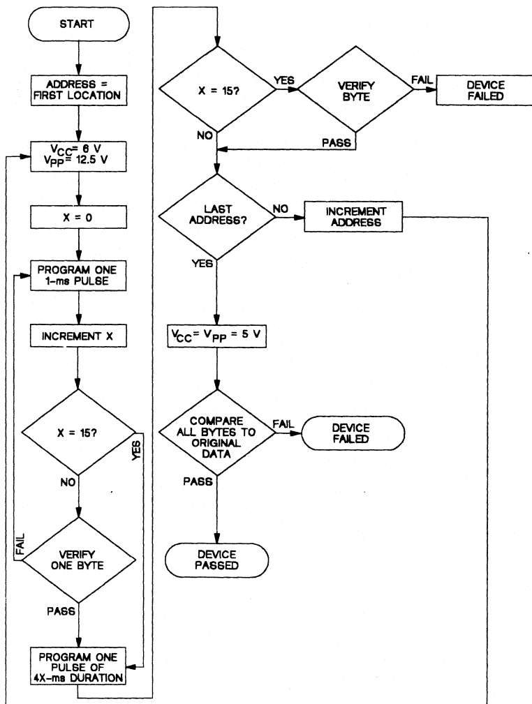
Figure G-3. Fast Programming Flowchart
