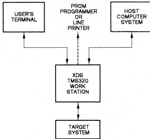
Figure E-3. TMS320C1x XDS/22 System Configuration
