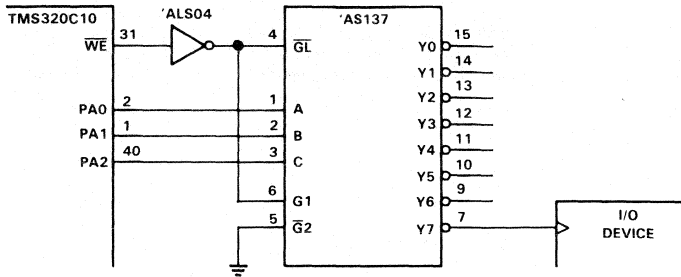
FIGURE 6. I/O DECODE CIRCUIT
